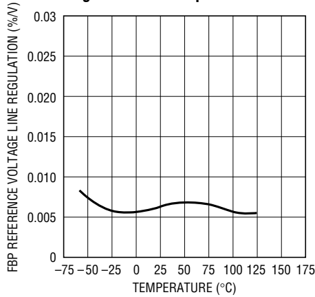
FBP Reference Voltage Line Regulation vs Temperature
